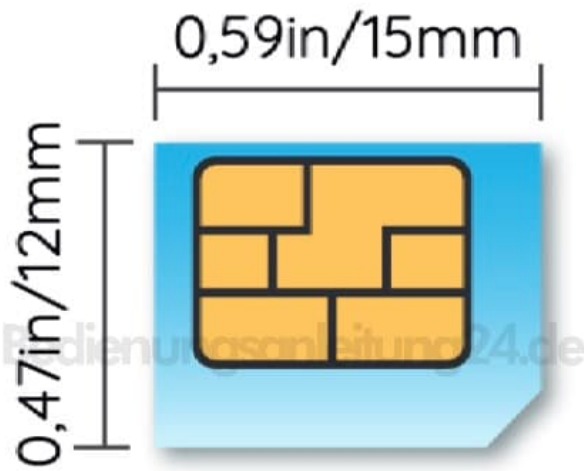
Micro-SIM /3FF (2004)
